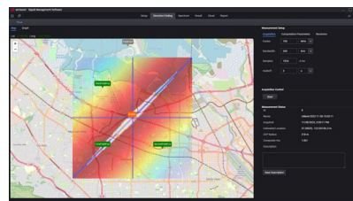
TDoA by three FieldFox
