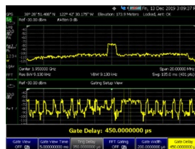
LTE FDD control channel captured with periodic frame trigger synced to GPS
